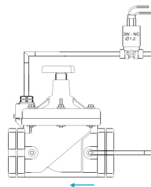
NO valve
