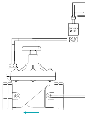
NC valve
